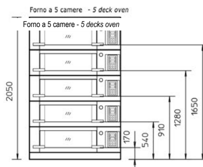
Forno con cella o basamento carenato (ruote optional) Oven with proper or base-box (castors optional)
